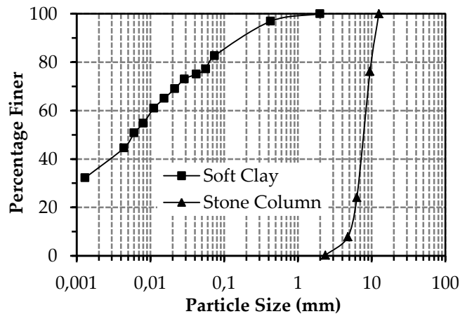
Figure 2. Particle size distribution for stone column and clay materials
