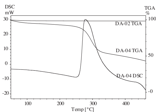
Figure 4. DSC and TGA thermograms of the materials.
