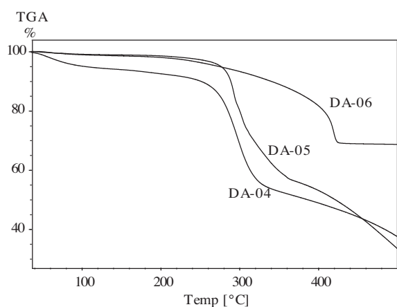
Figure 3. TGA characterization of the materials.
